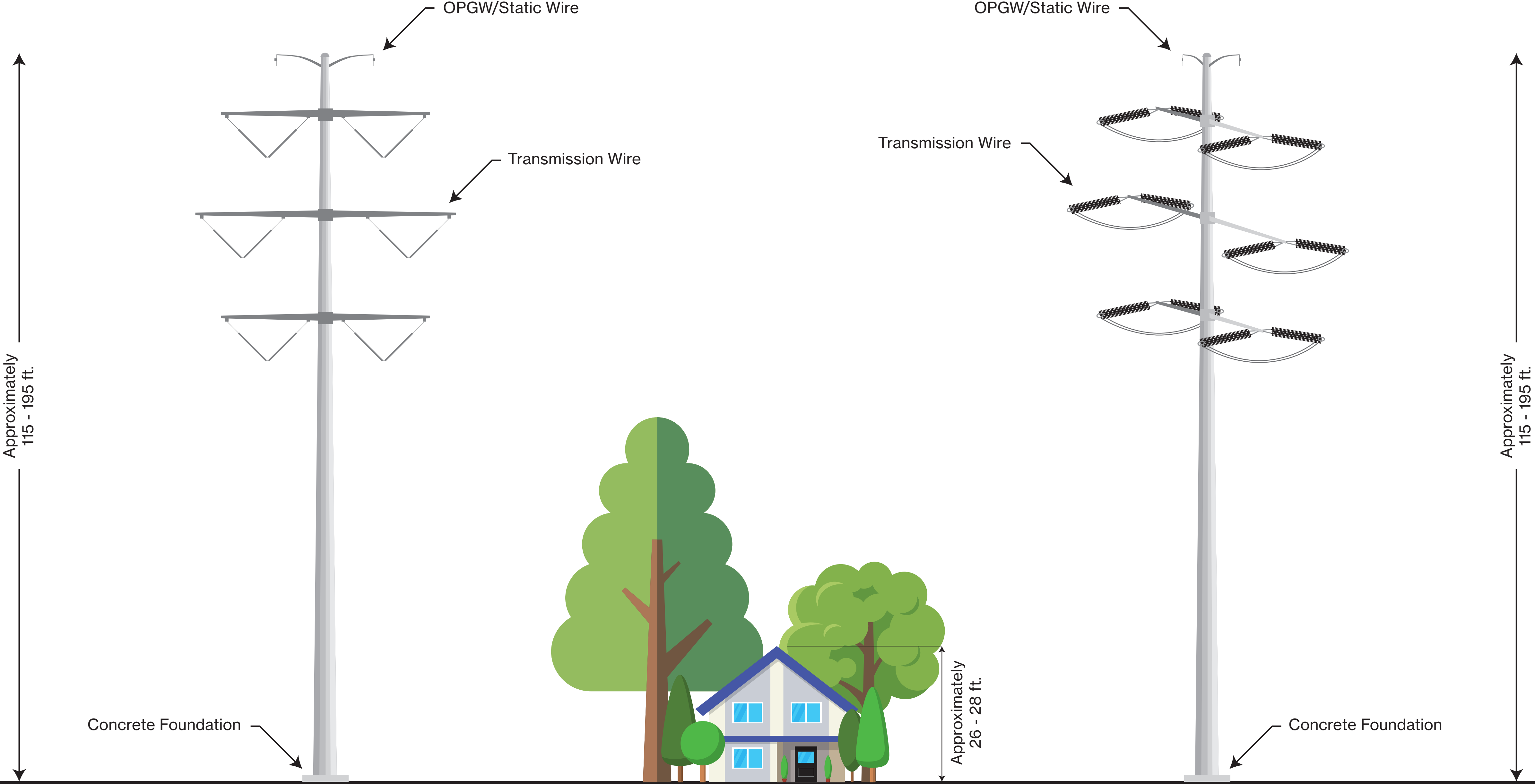
Steel Non-Angle Structure on Foundation
